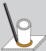
Pipe: Pipe axis: ASME: 2F fixed vertical
