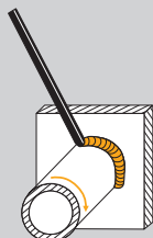
PB Pipe: Pipe axis: ASME: 2FR rotated horizontal
